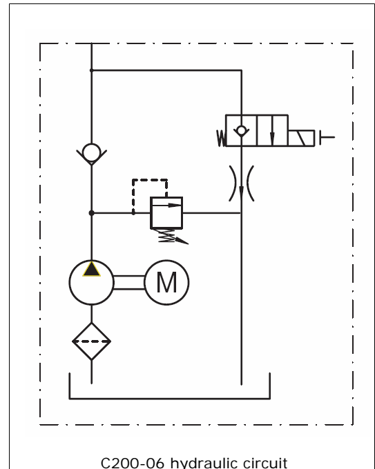
C200-06 hydraulic circuit
